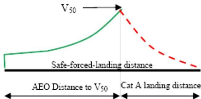
Figure 10 Category B (V50) safe-forced-landing distance
