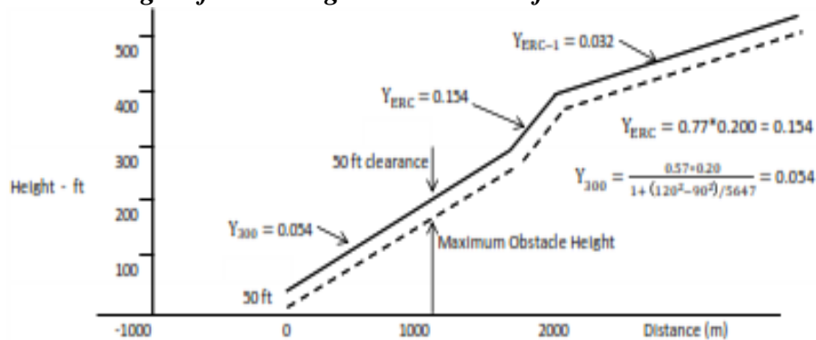
Figure 3 Assumed engine failure height less than 200 ft
