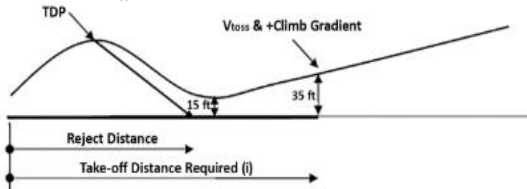
Figure 1 Clear Area take – off
