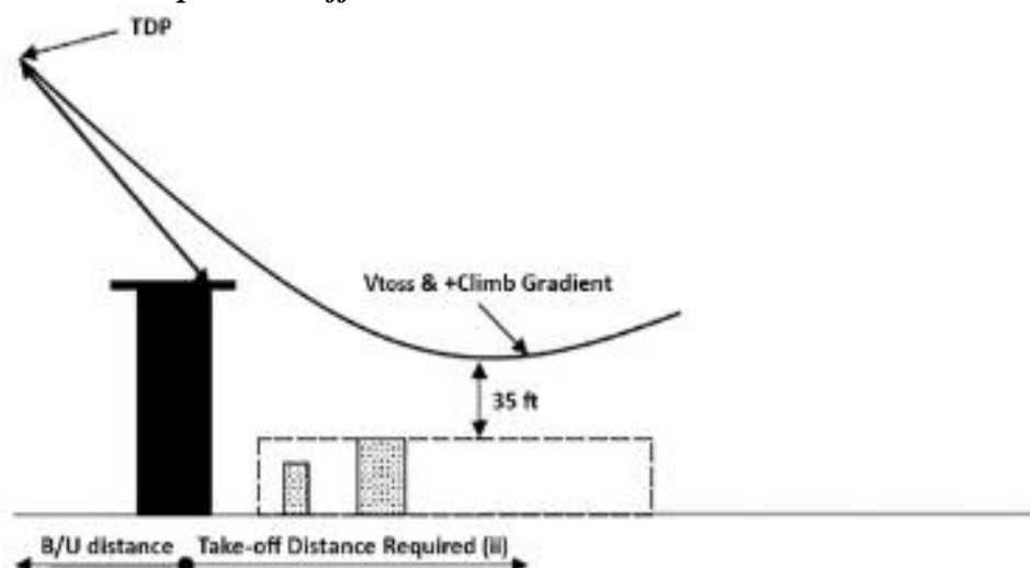
Figure 4 Elevate Helipad take-off
