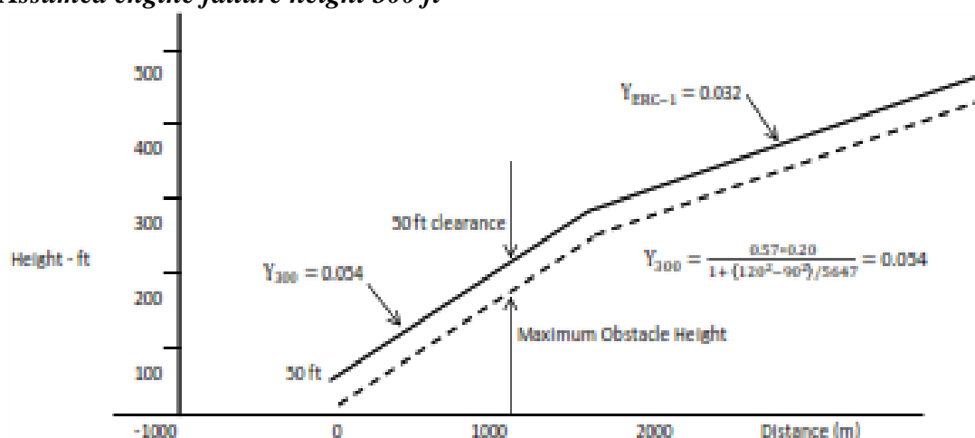
Figure 1 Assumed engine failure height 300 ft
