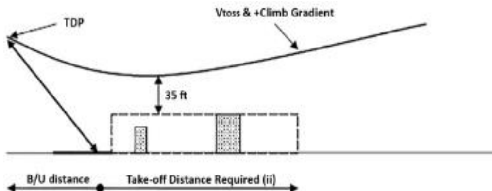
Figure 3 Helipad take-off
