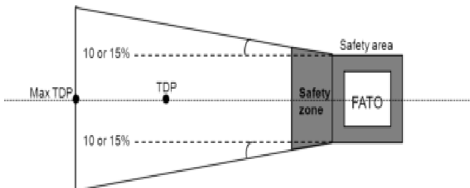
Figure 2 Obstacle accountability
