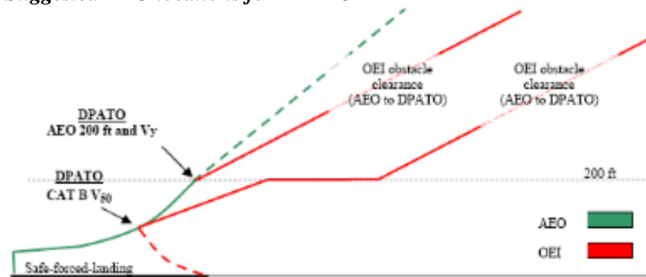
Figure 7 Suggested AEO locations for DPATO
