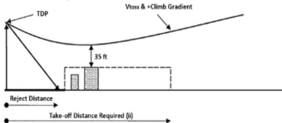
Figure 2: Short Field take-off
