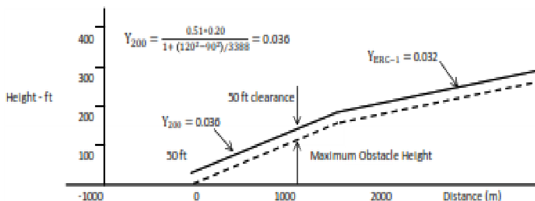
Figure 2 Assumed failure height 200 ft
