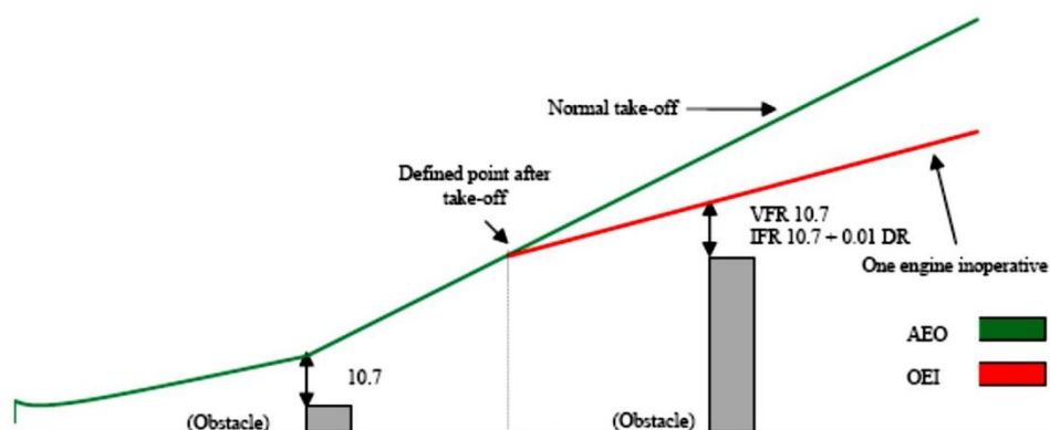
Figure 3 Performance Class 2 Obstacle Clearance
