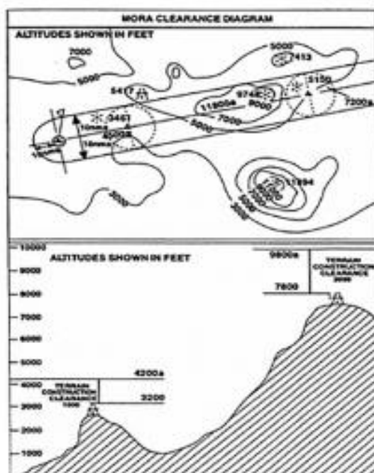
Figure 3 Jeppesen formula
