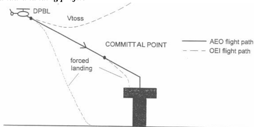
Figure 2 Standard landing profile
